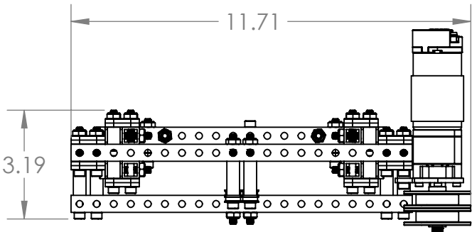
FULLY RETRACTED
