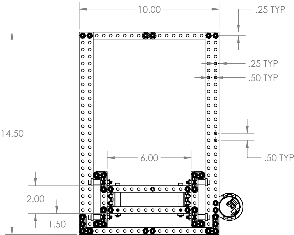
FULLY RETRACTED
