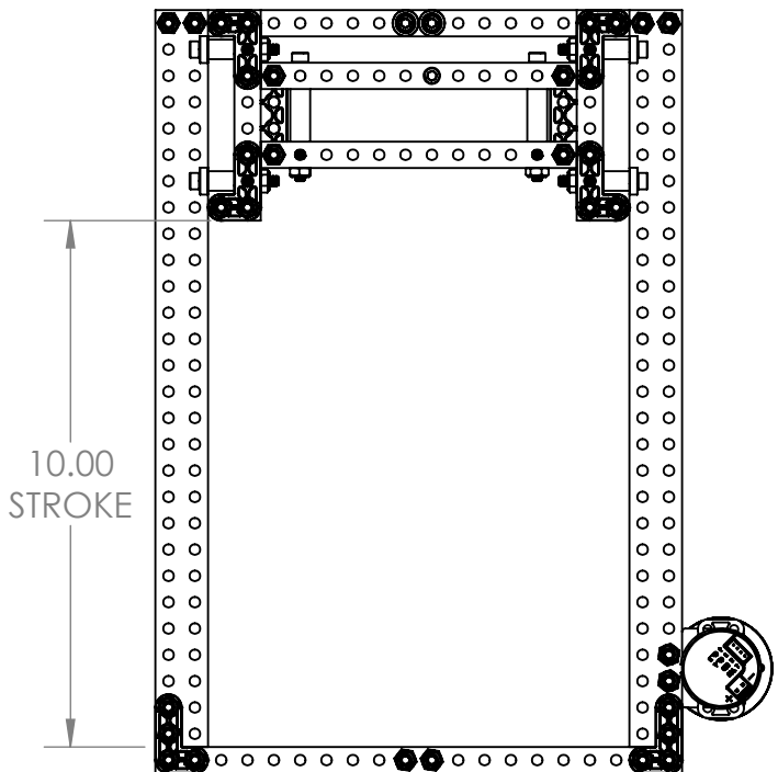
FULLY EXTENDED
